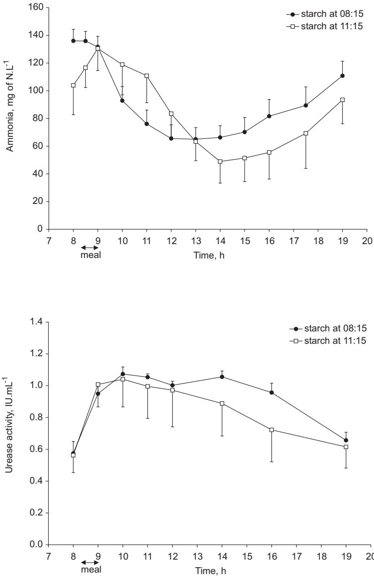
Figure 1. Effect of the time of starch supply on the variations in rumen ammonia concentration, and urease activity. Values are means of four sheep \pm SE.
